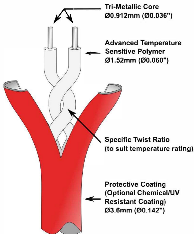
Figure 1: Fixed Temperature Linear Heat Detection Cable Construction
