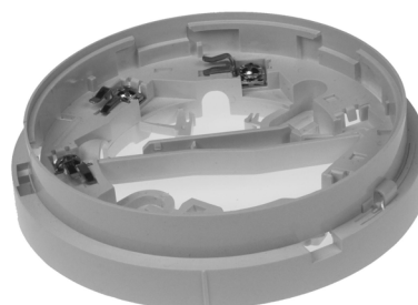
4098-5260 4" Continuity Base
